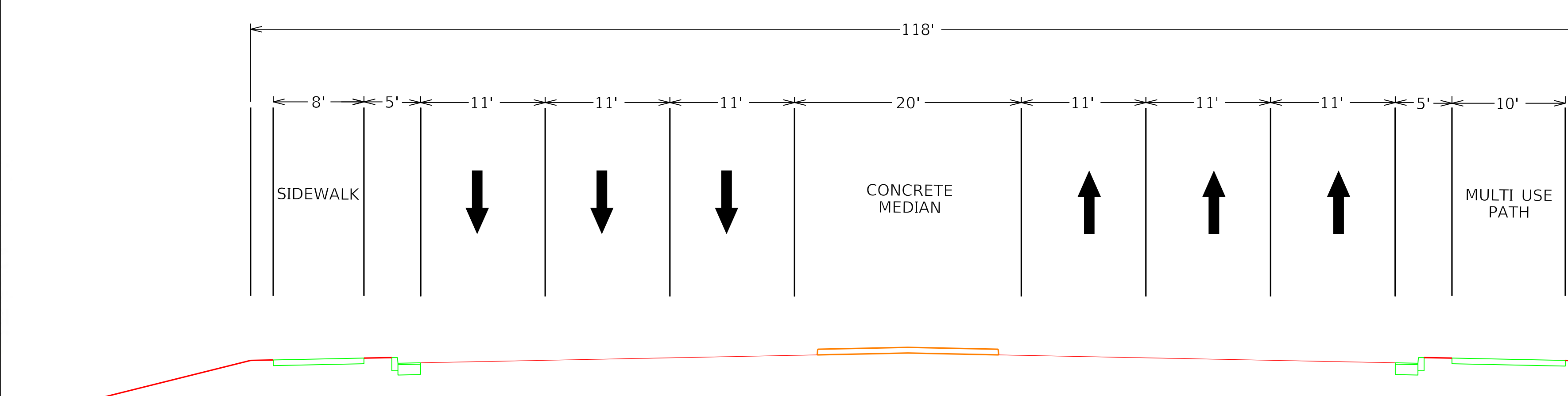
NEW CIRCLE ROAD TYPICAL 6 LANE OPTION
